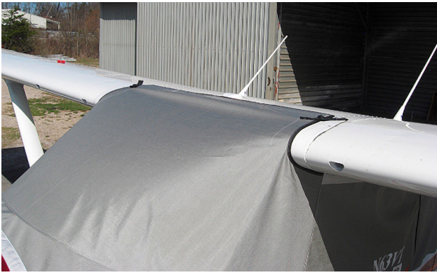
Standard Cessna 182 Canopy Cover Install Detail
