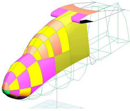
Schweizer 2-33A Canopy/Nose Cover, 3D model
