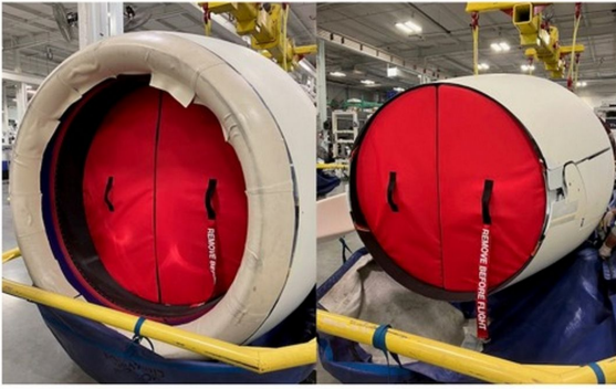
INLET & THRUST REVERSER FOD PREVENTON PLUGS/COVERS
