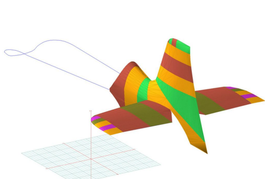
Gamebird GB-1 Empennage Cover, 3D model
