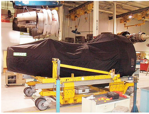
GE CF-6 QEC Engine Long-term Storage/Transport Cover "Bag" (Boeing 767)
