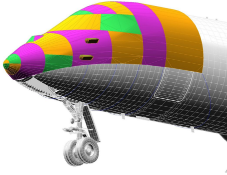
Bombardier Global Express Cockpit/Nose Cover, 3D model
