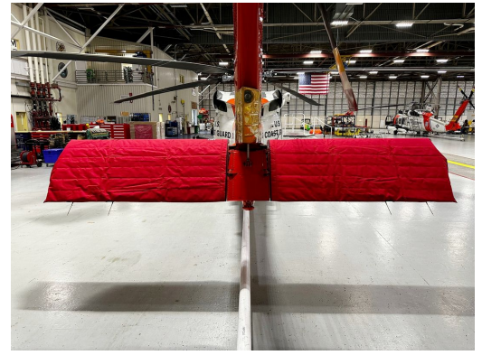
Sikorsky Blackhawk Horizontal Stabilizer Covers, Padded for maintenance protection U.S. Coast Guard MH-60 Padded Horizontal Stabilizer Covers
